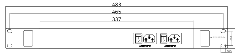
Rear View
