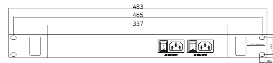
Rear View
